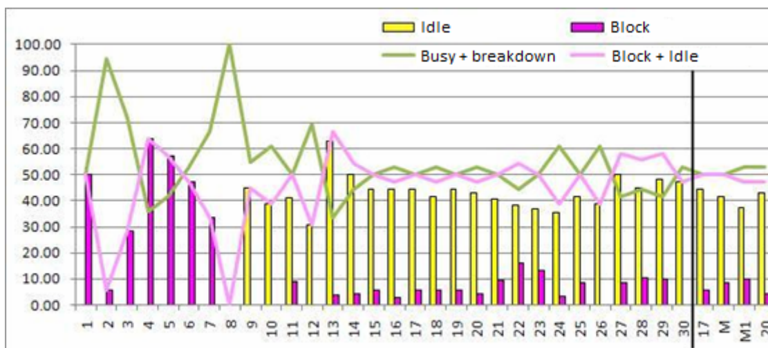
Figure 8. Result of the bottleneck analysis using the Turning point method
