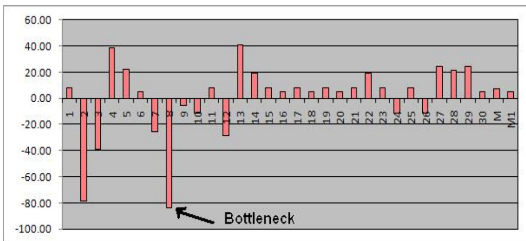
Figure 10. Results of the bottleneck analysis using the Criticality indicator based method
