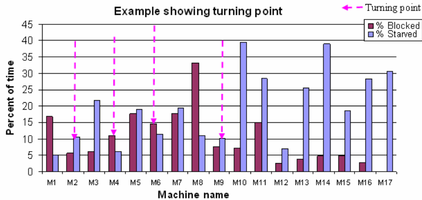
Figure 2. Example of turning points determination
