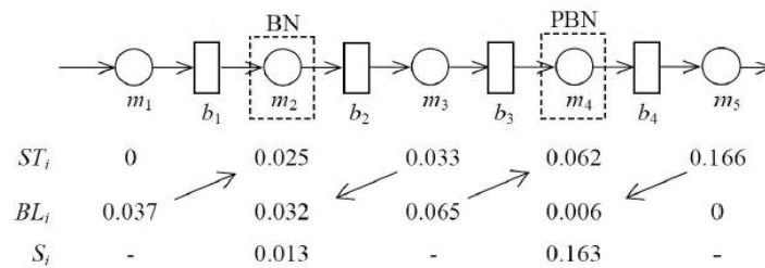
Figure 3. Example of the bottleneck identification in the open serial line
